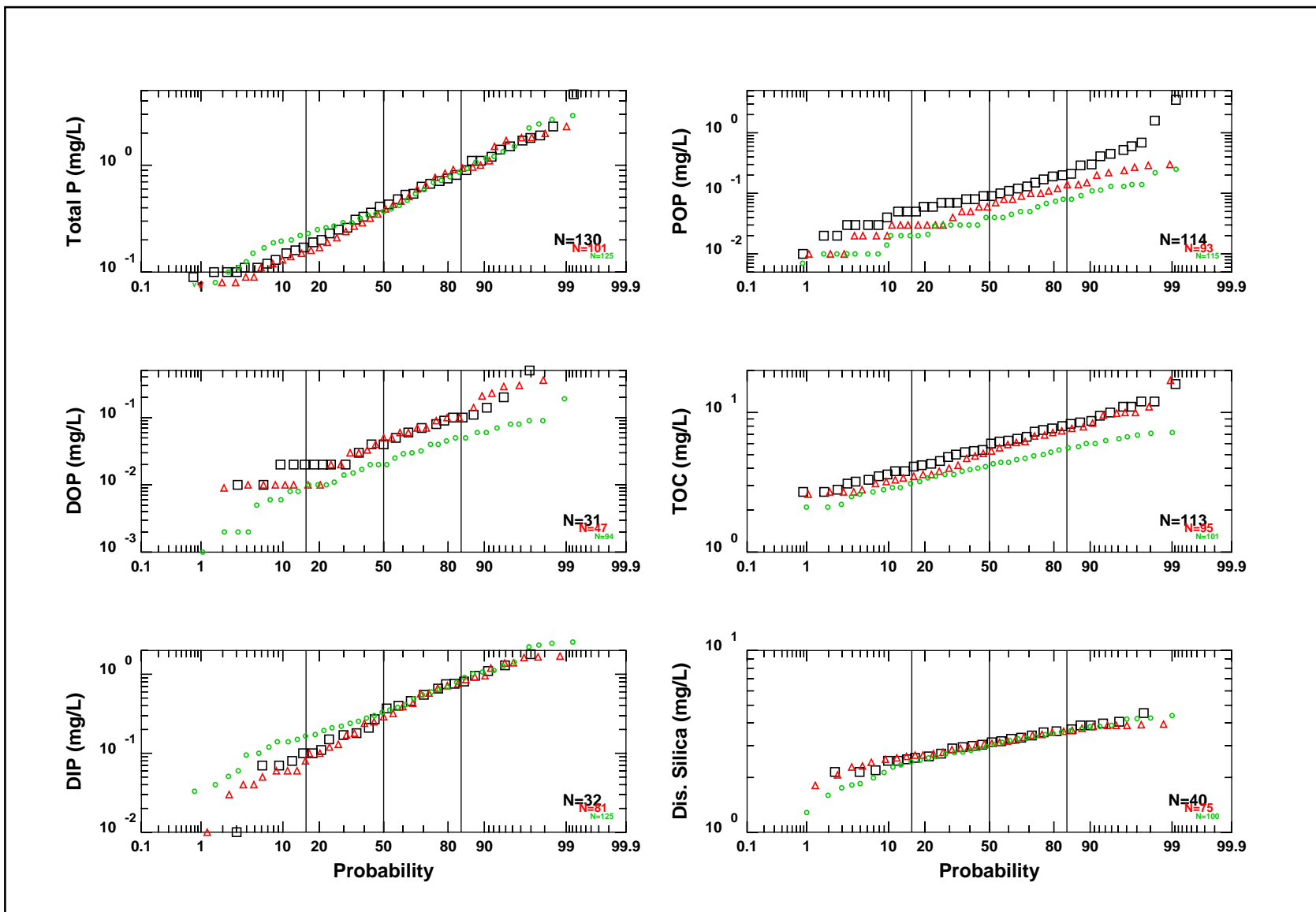
Probability of Fall-Line Concentration and Flow, Naugatuck River at Beacon Falls, CT.
